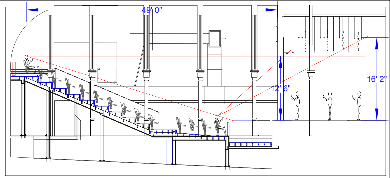
PLAYHOUSE THEATRE CHELTENHAM BASIC SIDE ELEVATION
